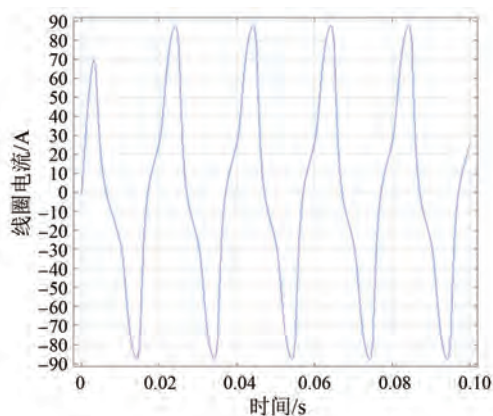
图 11 匝间短路时二次侧故障相非故障匝电流波形 Fig. 11 Current waveform of the non-faulted turns in the faulty phase on the secondary side during an inter-turn short circuit fault
